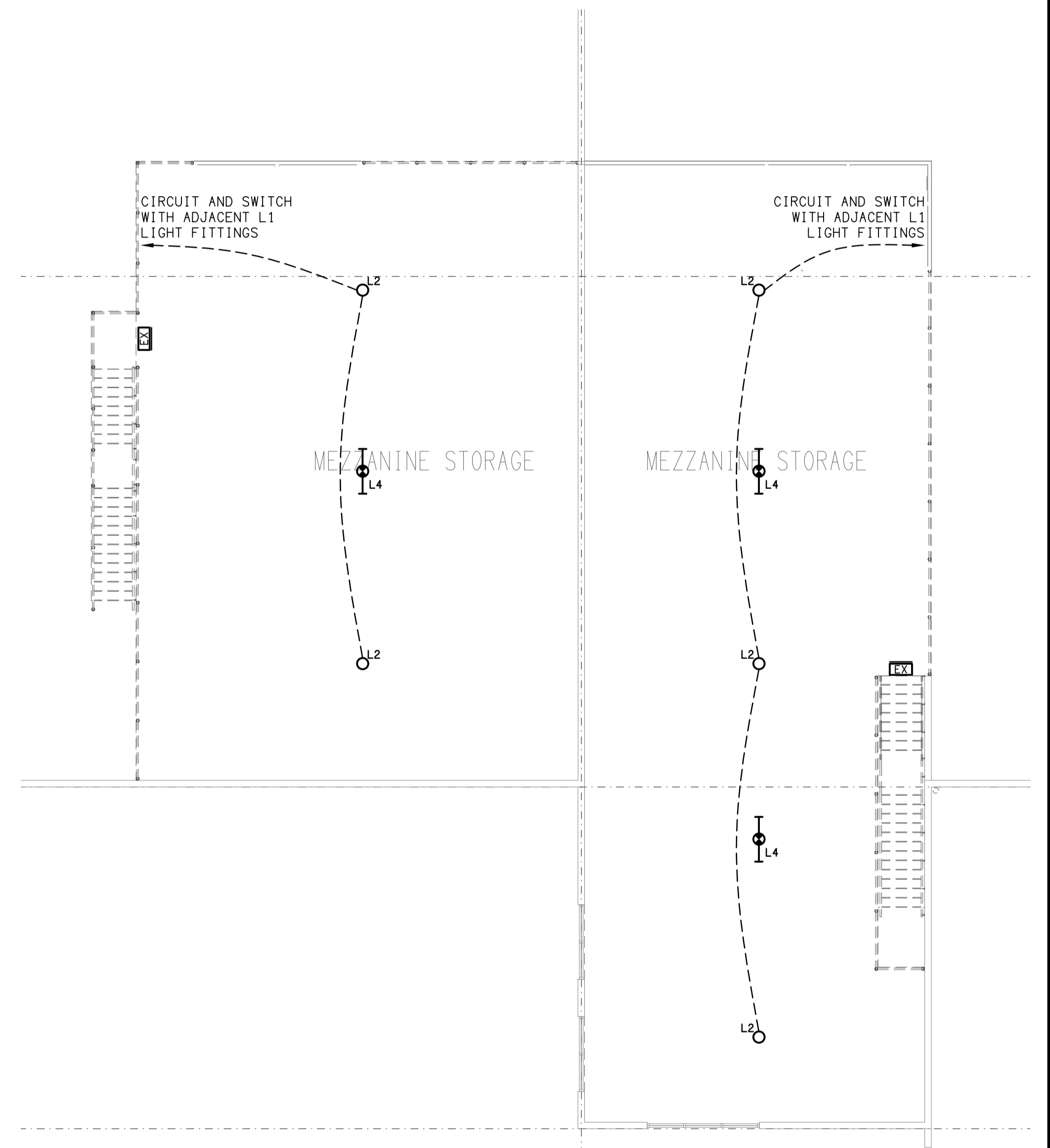
LEVEL 1 REFLECTED CEILING PLAN SCALE 1: 100
